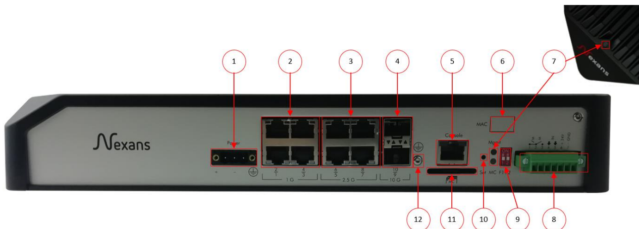
Figure 5: Interfaces of XGigaSwitch DICE 8TP 2SFP+ DC
