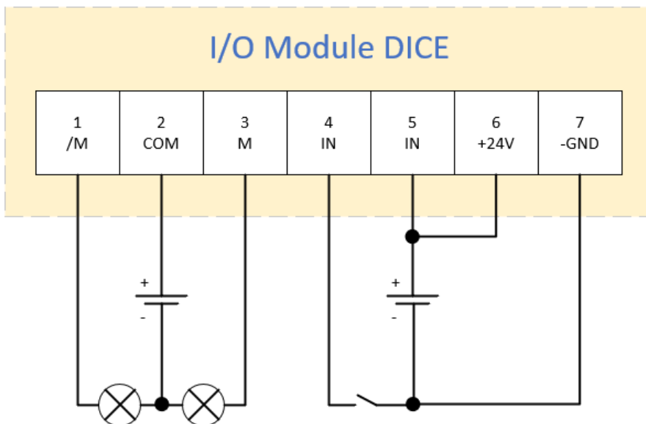
Figure 16: Connection plan of the I/O ports
