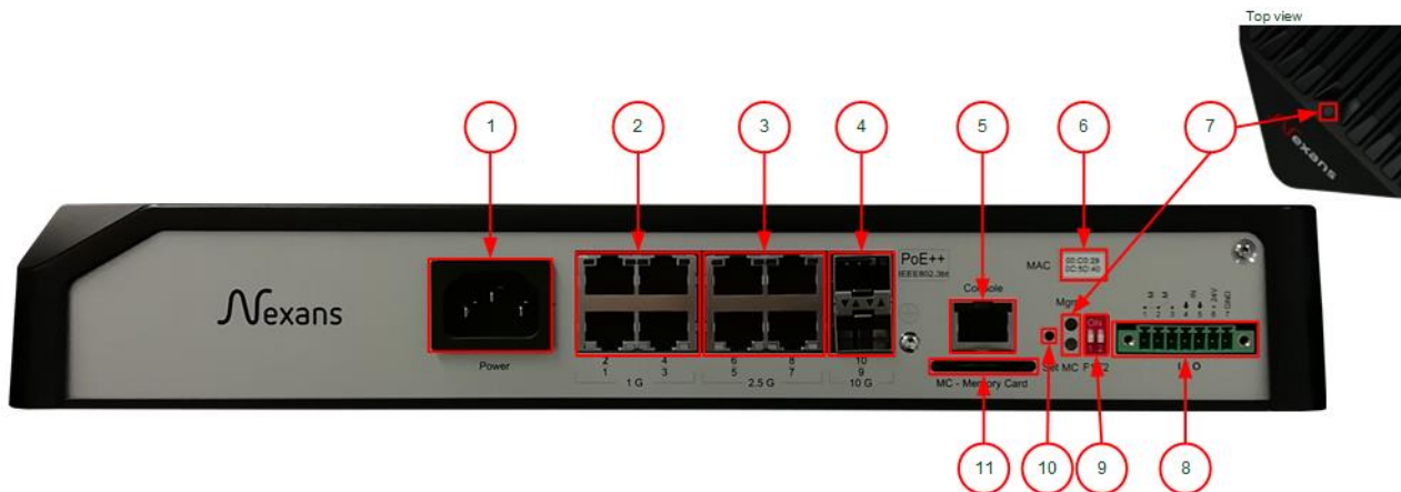
Figure 4: Interfaces of XGigaSwitch DICE 8TP 2SFP+ AC
