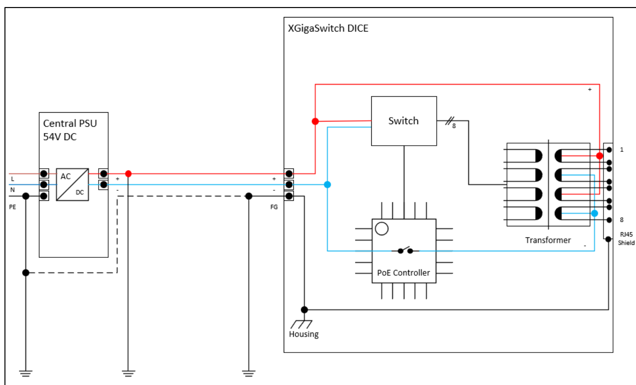
Figure 14: Block diagram of grounding
